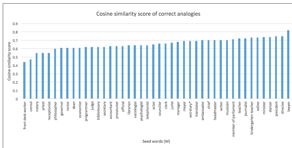
Figure 1. Cosine similarity score for correct female analogies for male occupation seed words 4 .
